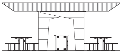
② Side View 1 : 50
