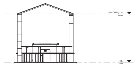
③ Front / Back View 1 : 50
